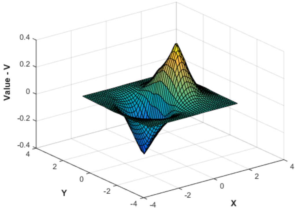
Interpolation of v = x \cdot \exp(-x.^2 - y.^2) with sample points removed
